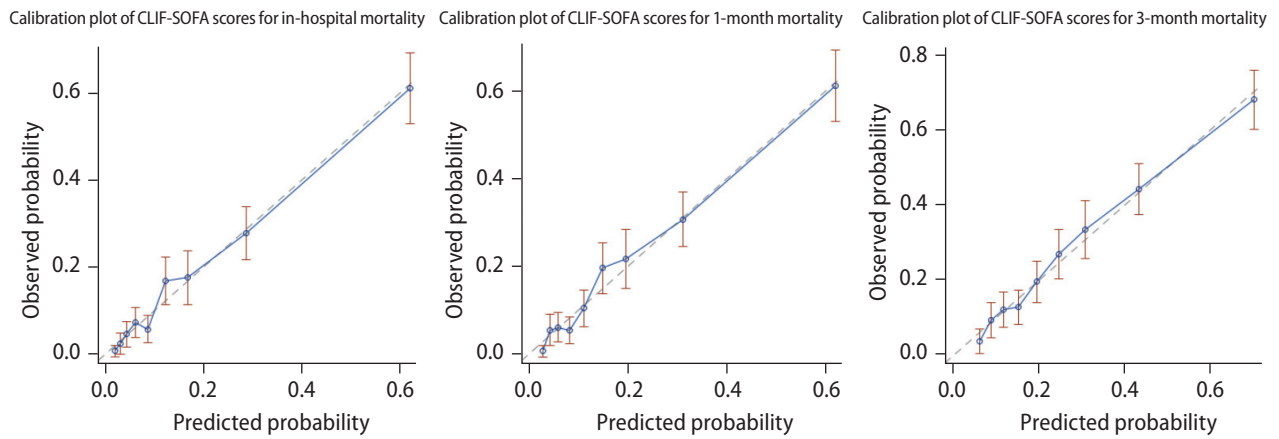
Supplementary Figure 1. Calibration plot of CLIF-SOFA scores. Diagonal line is the line of perfect calibration. Dots represent the intersects of observed and expected values for the risk of mortality, and bars represent the 95% confidence interval of the observed probability. Blue line indicates the calibration trend; since this line is close to the diagonal line, it indicates that the CLIF-SOFA fits the data well. CLIF-SOFA, Chronic Liver Failure-Sequential Organ Failure Assessment.
