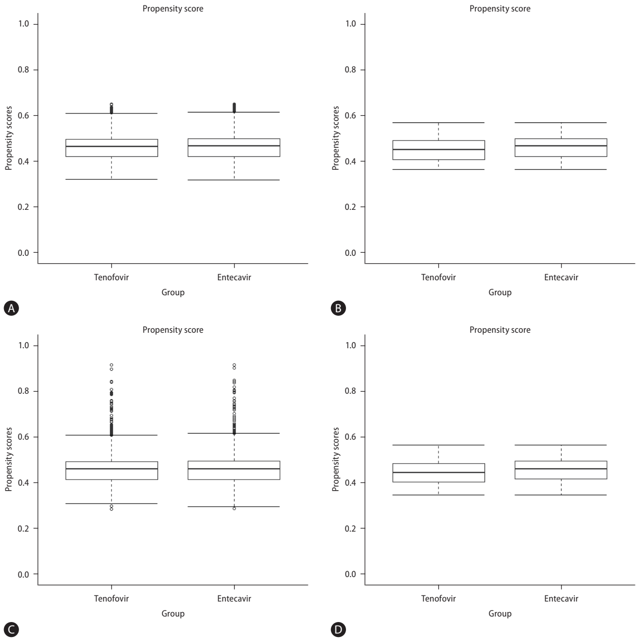
Supplementary Figure 1. Distribution of propensity scores. Propensity scores of the entire study population after (A) PSM and (B) IPTW and those of the NHIS Health Check-Up Database subcohort after (C) PSM and (D) IPTW. IPTW, inverse probability of treatment weighting; PSM, propensity score matching.
