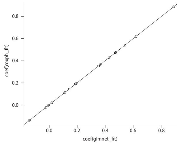
Supplementary Figure 1. Calibration plot of coefficients of ML-based score and coefficients of Cox-based score.
