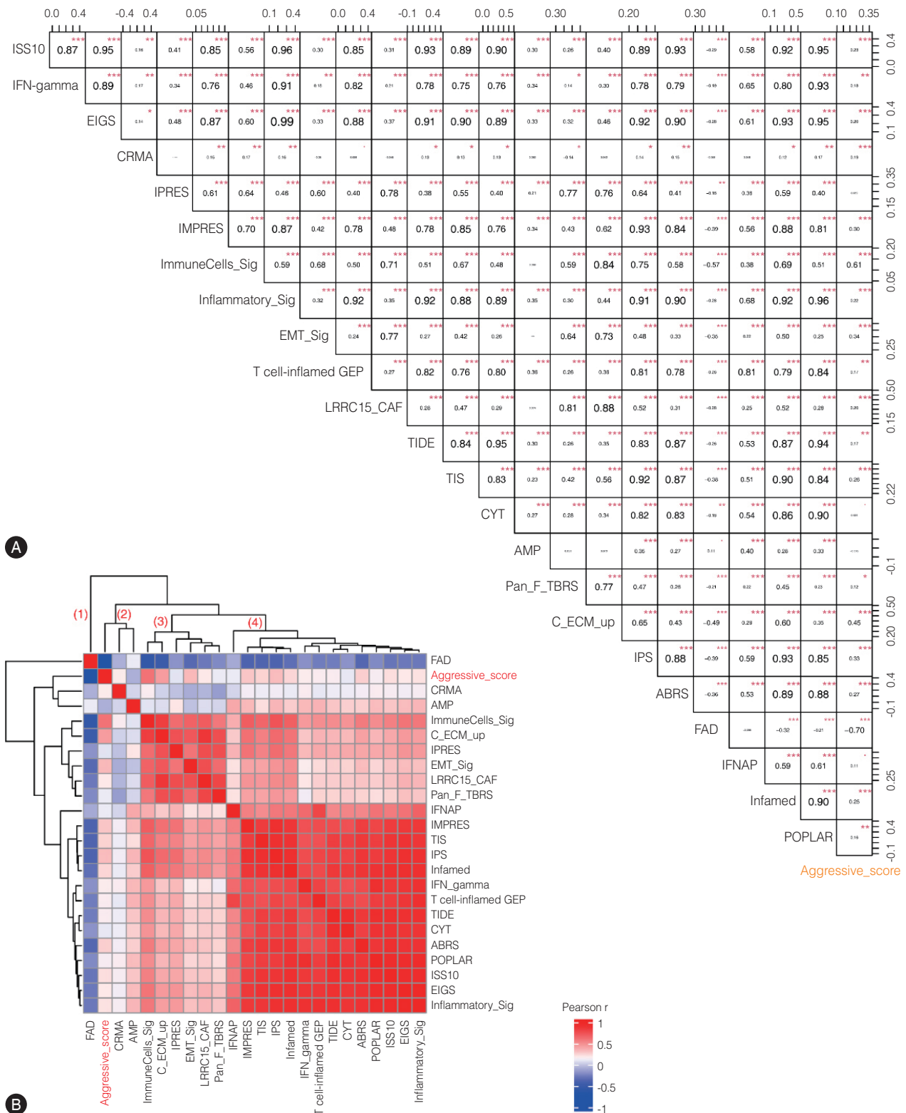
Supplementary Figure 2. The correlations between 23 previously curated immunotherapy response predictive signatures and the aggressive score, as represented by a correlation matrix (A) and a heatmap (B). In panel (A), the numbers denote Pearson's correlation coefficients (r values), while the asterisks indicate statistical significance: * P < 0.05 ; ** P < 0.01 ; *** P < 0.001 . In panel (B), four clusters were identified.
